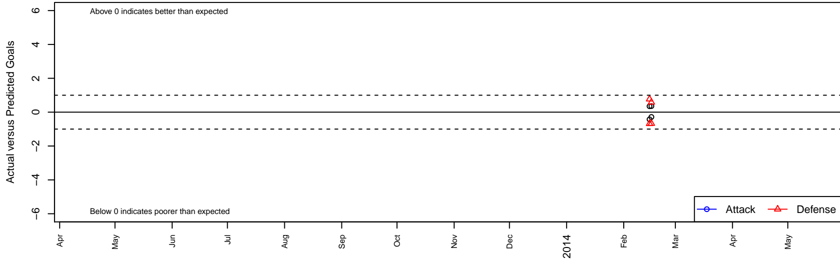
Arsenal Colorado 99-00 Gold B99 Dots are actual minus expected GF (blue circles) and GA (red triangles). Blue line is smoothed change in attack strength. Red is smoothed change in defense strength.
